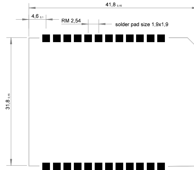
Solder pads description
