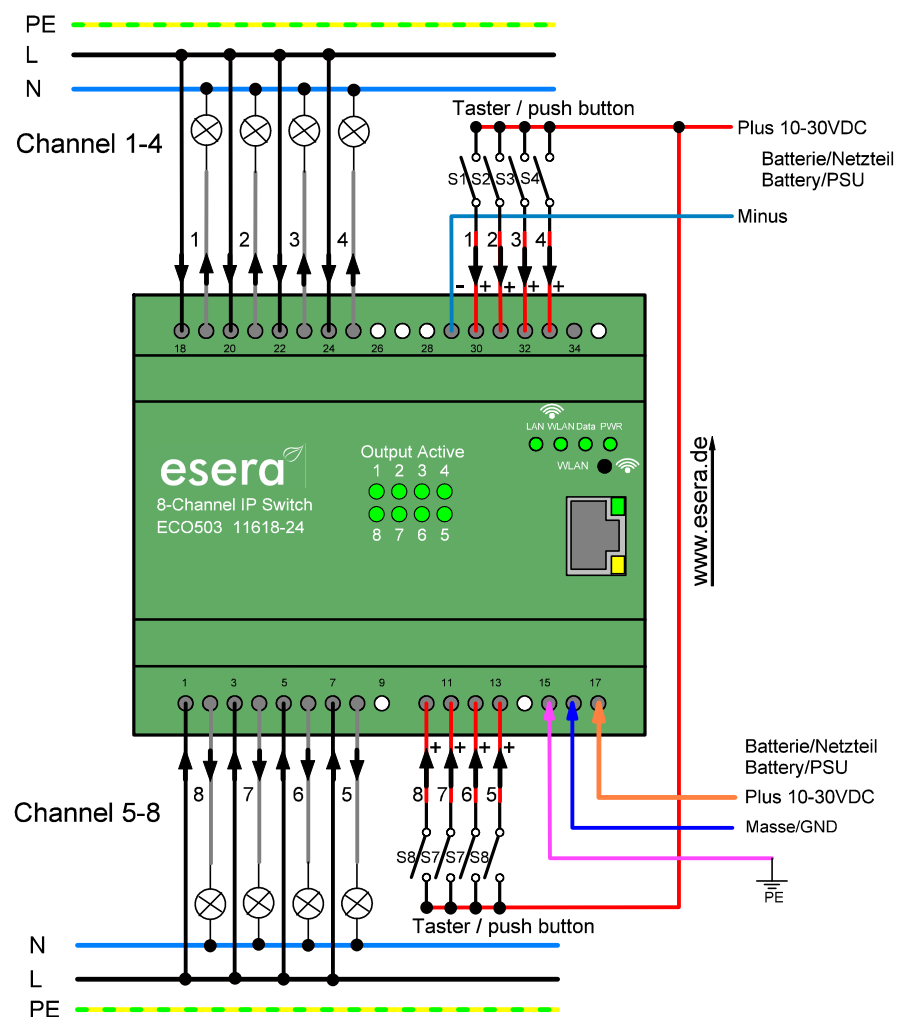
8-Channel Switching Actuator
